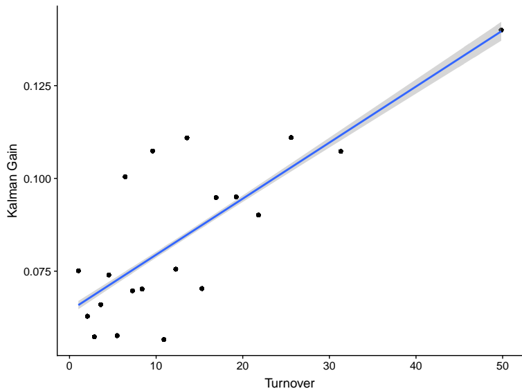
Figure 6: Distribution of Kalman gains across turnover
