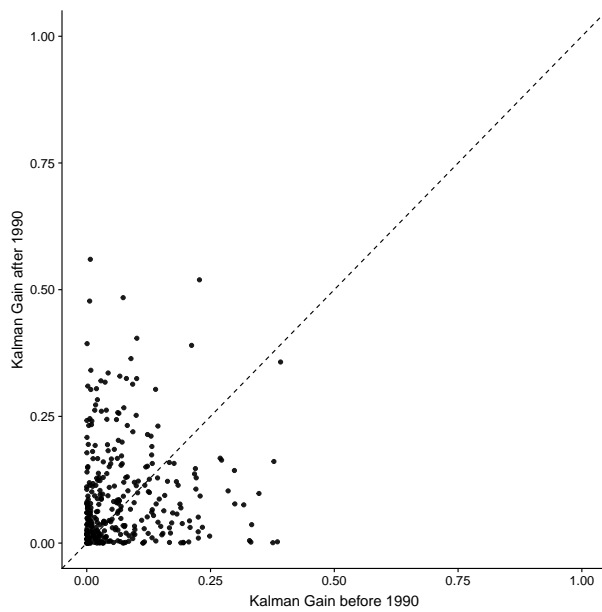
Figure 8: Kalman gains for individual stocks pre- and post- 1990
