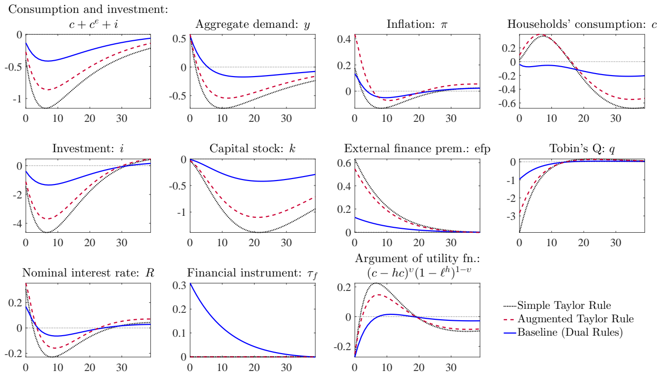
Figure 4: Impulse Response Functions to Risk Shocks
