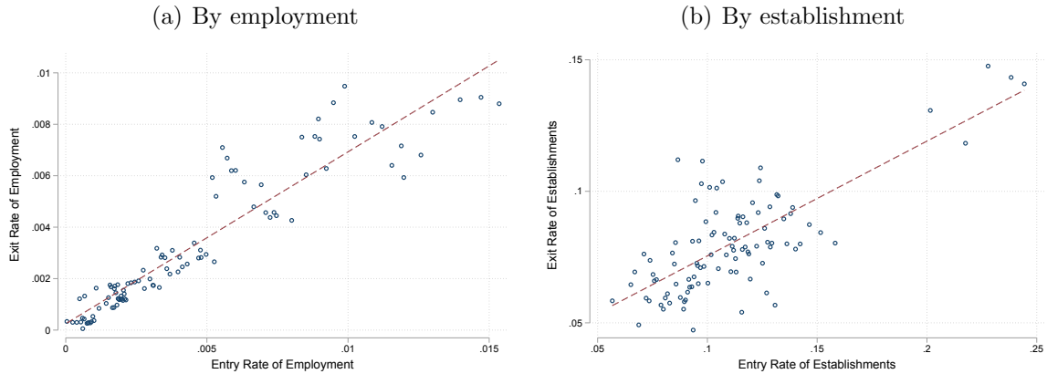
Figure A4: Correlation between entry and exit rates
