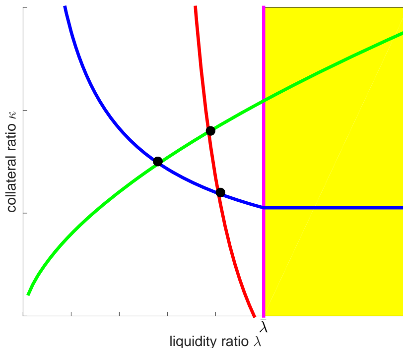
Figure 7: The red curve is equation (15)
