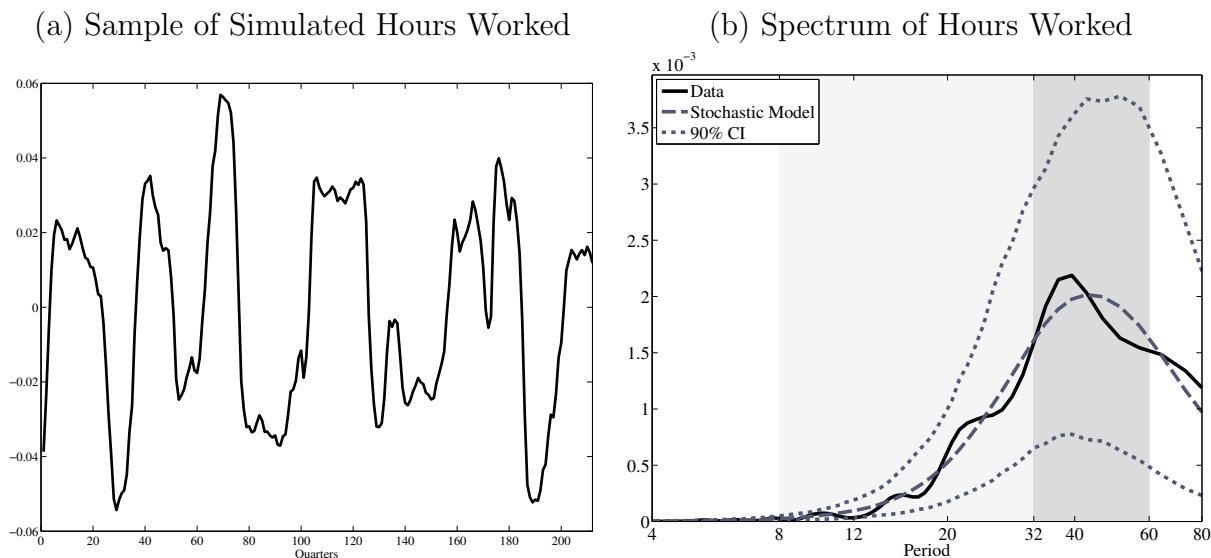
Figure 7: Stochastic Model
