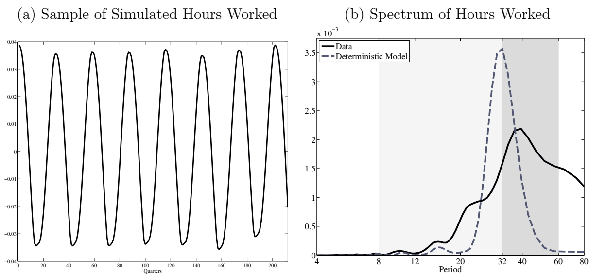
Figure 6: Deterministic Model
