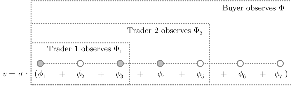
Figure 1: Example of information sets in trading network. The figure illustrates the information structure when two intermediaries are involved ( M = 2 ) in trading an asset whose common-value component v depends on seven factors \phi_i ( N = 7 ). The dotted rectangles indicate the set of factor realizations that are observable to the two intermediaries and to the expert buyer (remember: the firm/seller observes none of these factors). Factor realizations \phi_i \in \{0, 1\} are indicated by the circles that are either unfilled (for \phi_i = 0 ) or filled (for \phi_i = 1 ). The seller is uninformed and thus does not observe any of the factor realizations.
