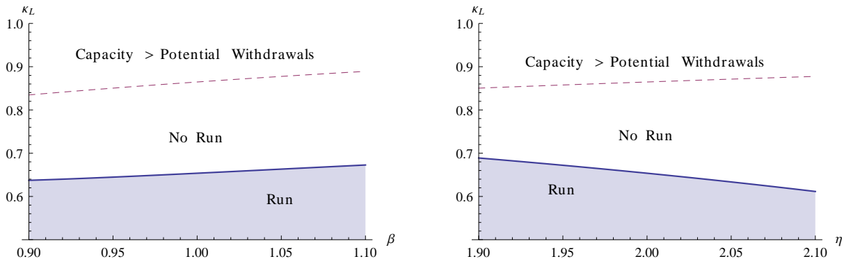
Figure 6: Minimal Capacity Required to Eliminate Runs
